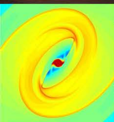
Numerical Simulation of Galaxies
